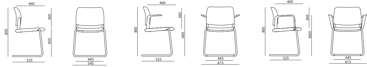
Fusto slitta Sled based without armrests Base trineo sin reposabrazos
