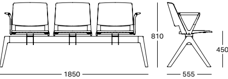
Panca 3 posti con gamba GP04 e braccioli REVOLUTION/70-71 3 seater bench with GP04 leg and REVOLUTION/70-71 armrests Banco de 3 plazas con pata GP04 y brazos REVOLUTION/70-71
